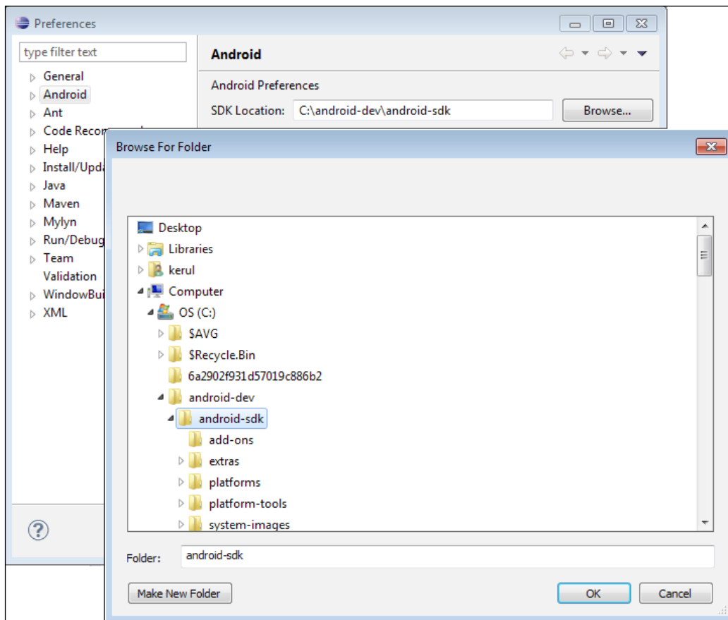
Android preferences in Eclipse
