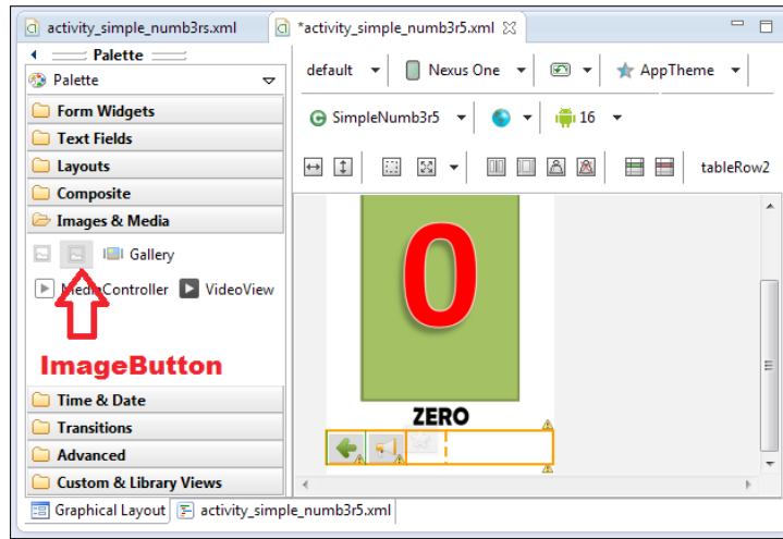
Adding ImageButtons
