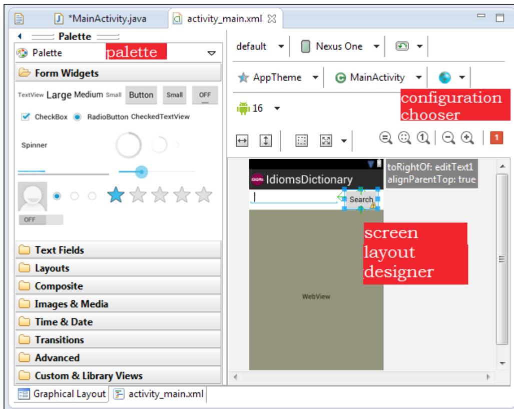
The ADT's GUI designer
