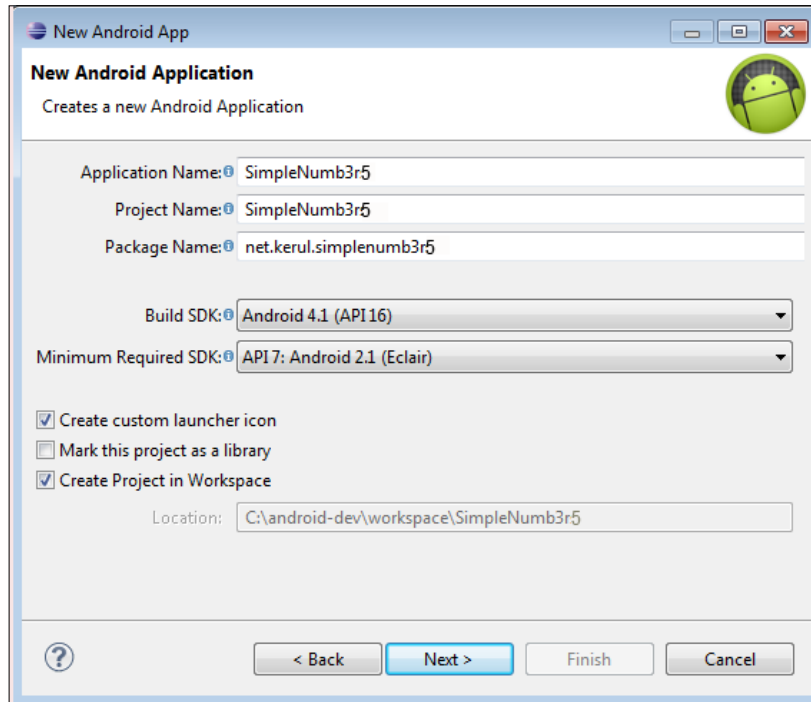
Create a new Android project named SimpleNumb3r5
