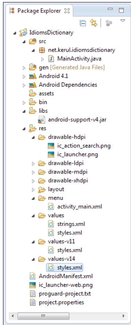
Project explorer
