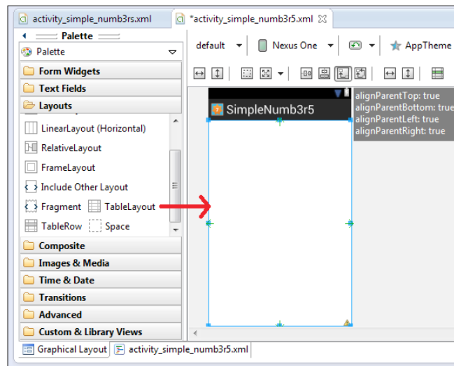
Inserting a TableLayout
