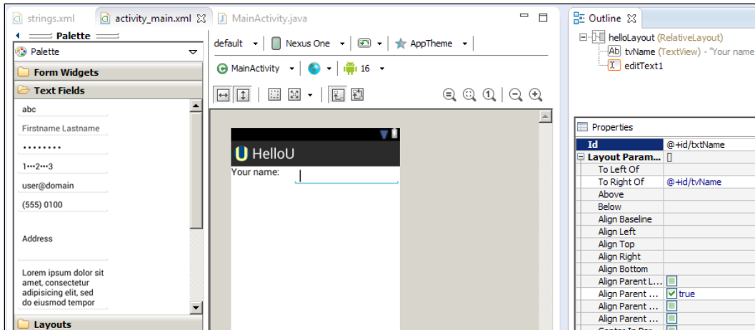
Adding an EditText
