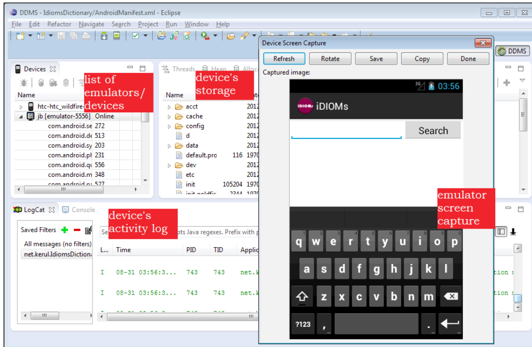
Dalvik Debug Monitor Server (DDMS)
