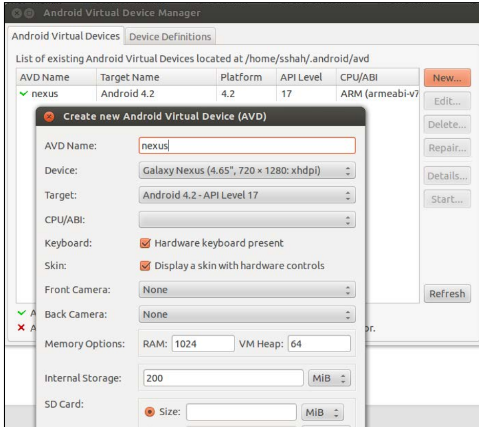
Creating a new AVD
