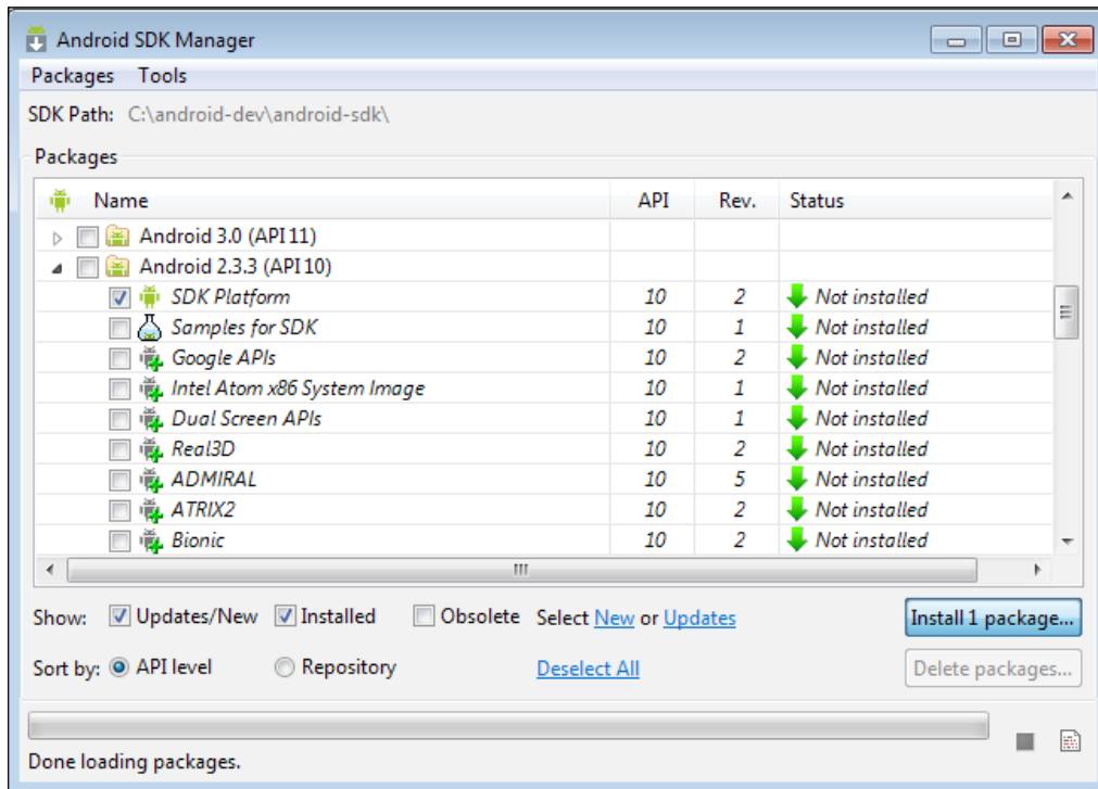
The Android SDK Manager window
